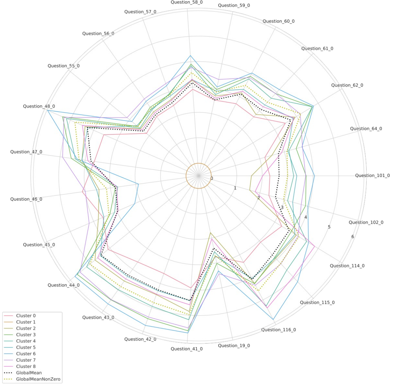
Star Plot for Whole Citizens Data
